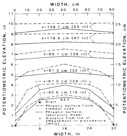
FIGURE 12. Three-dimensional finite-element results versus potentiometric elevations from Kenney, Pazin, and Choi (7): 69-cm (27-in) drains, 81.3-cm (32-in) spacing.
