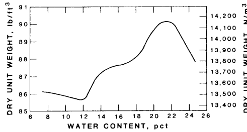
FIGURE 4. Moisture-density curve for sand used in laboratory model.
