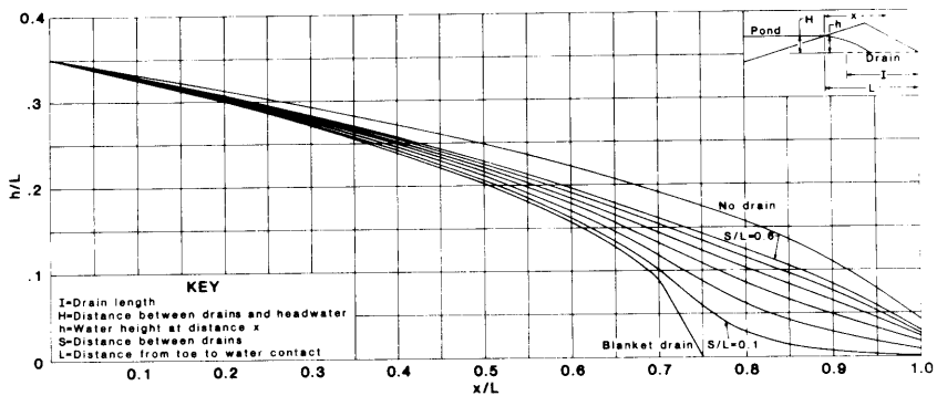
FIGURE 16. Dimensionless phreatic profiles, H/L = 0.35 , I/L = 0.25 .
