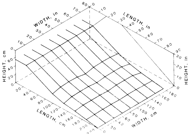
FIGURE 8. Potentiometric data for laboratory embankment model: Drains 1, 5, and 9 inserted at 1.83 m (6 ft), headwater = 49.3 cm (19.4 in).
